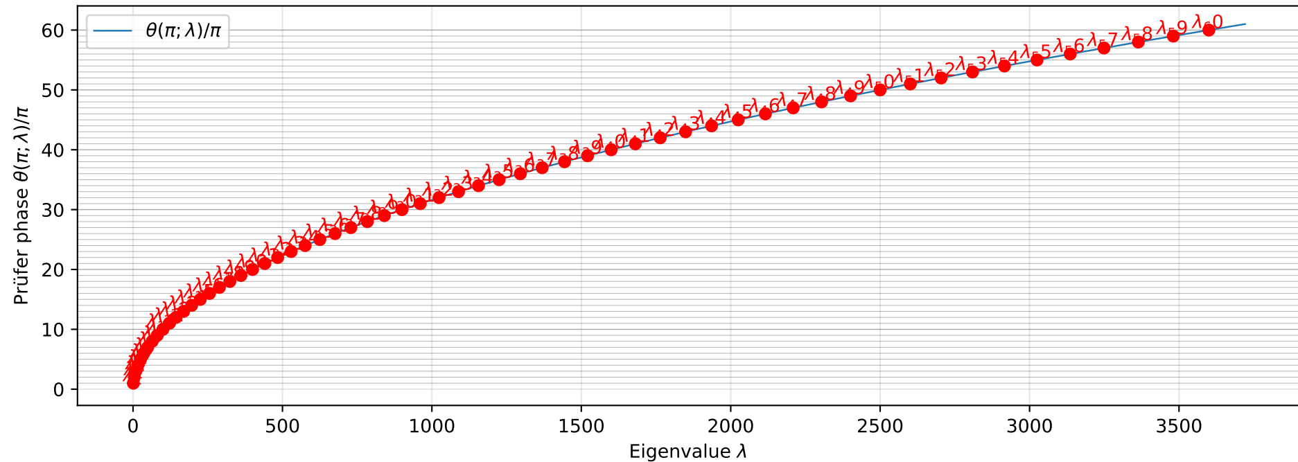
Prüfer phase sweep on clustered grid (n=100, 70%/30%) for 60 eigenvalues
